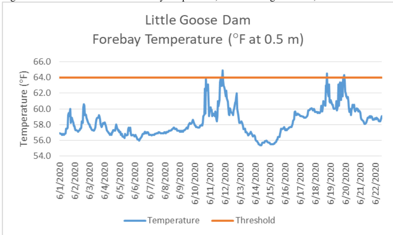
Figure 1: Little Goose 0.5 meter forebay temperature; June 1 through June 22, 2020.
